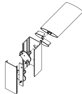
Fin fixation to the vertical frame profile
