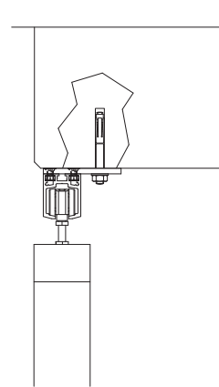
Flush-fixation
