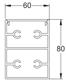
Horizontal top and bottom frame profile
