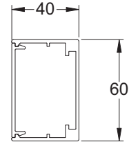
Vertical frame profile
