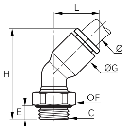
racor orientable
