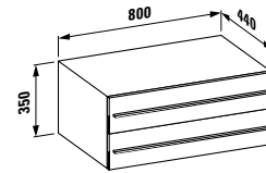
Consola mural de 2 cajones. 4.2023.4.080.525.1
