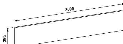
Espejo 2000 x 350, aluminio. 4.4030.5.080.007.1
