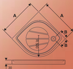
ELIPSO PRO 80 A = 800 mm ELIPSO PRO 90 A = 900 mm ELIPSO PRO 100 A = 1000 mm B = 200 mm
