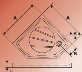
GENTA PRO 90 A = 900 mm B = 200 mm
