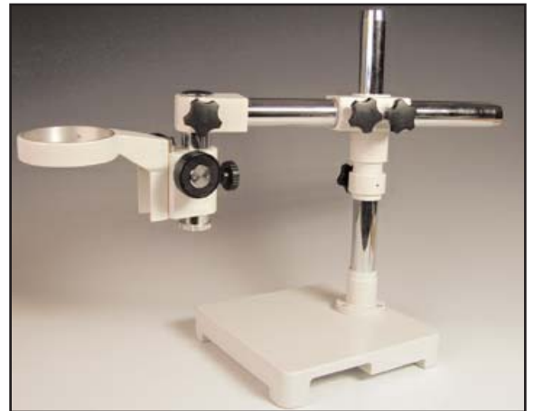
Plain stand with verticle and horizontal posts plus rack and pinion focusing mount.
