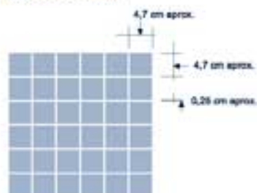
Mosaico 5x5 cm 12"x12" 30x30 cm (29,75x29,75 cm)
