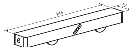
Tándem Regulable C-90106-03-0-1
