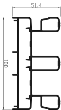
Ref. 21055 Marco tres carriles perimetral
