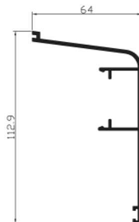
Ref. 16073 Tapeta guía superior corredera
