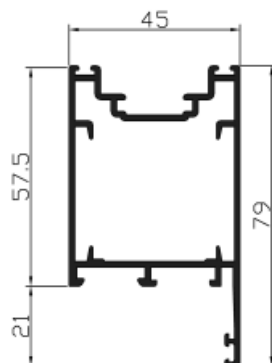
Ref. 24547 Hoja vaivén * Consultar stock
