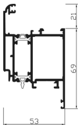
Ref. 22741* Hoja balconera
