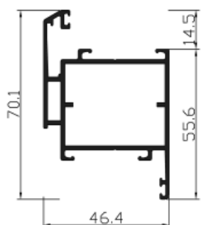
Ref. 26195 Perfil puerta practicable
