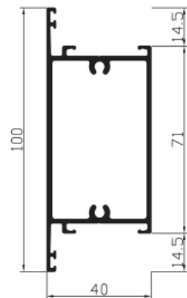
Ref. i9739 Travesaño 100 mm
