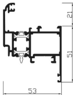
Ref. 22739* Hoja ventana
