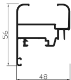
Ref. 21363 Hoja ventana
