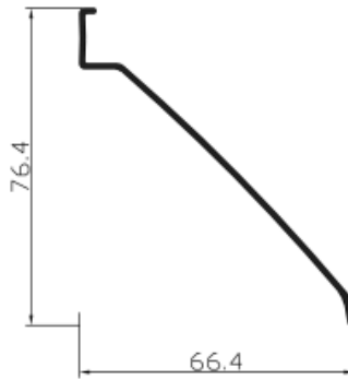
Ref. R270 Lama fija
