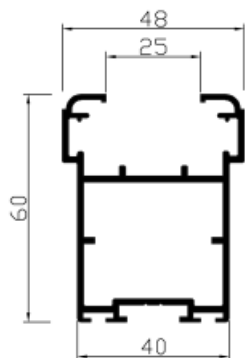
Ref. 2517 Hoja corredera / plegable
