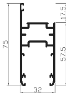
Ref. 21059 Hoja ajunquillada
