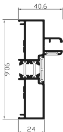
Ref. 22404 Marco lateral 90 mm
