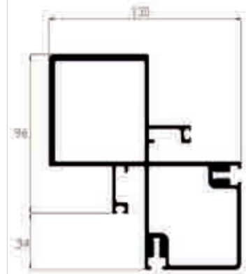
Ref. 21124 Esquinero
