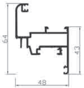
Ref. 27030 Hoja ajunquillada
