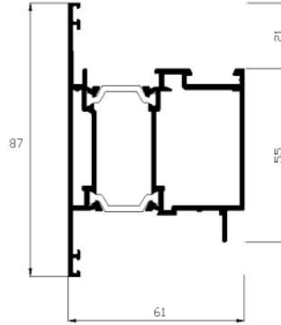
Ref. 22461 Hoja apertura exterior *Consultar stock
