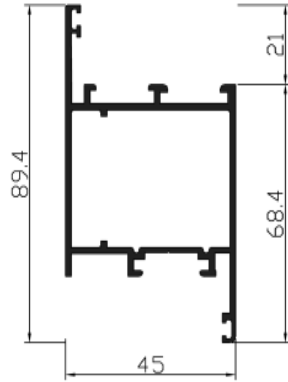
Ref. 21642 Hoja balconera
