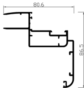
Ref. 121692 Semi marco interior
