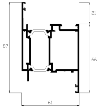
Ref. 22460 Hoja apertura interior *Consultar stock
