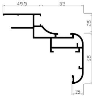
Ref. 121582 Semi marco interior
