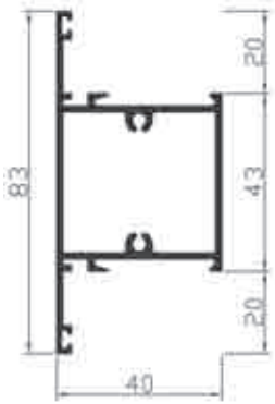
Ref. 19636 Travesaño
