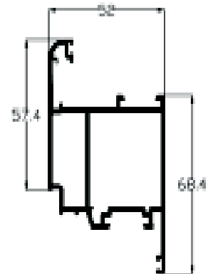
Ref. 24543 Hoja balconera
