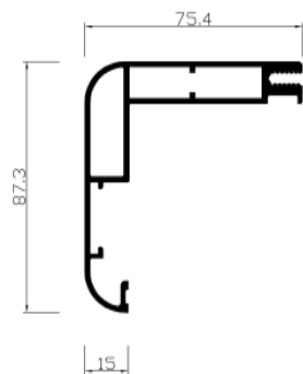
Ref. 121681 Semi marco exterior
