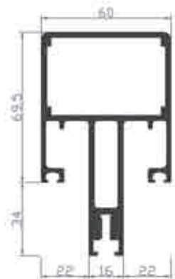
Ref. 21130 Montante
