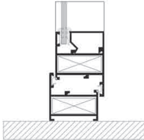
Practicable Samblex 40i
