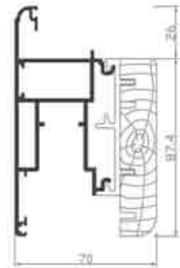
Ref. 21914+7L0 Hoja corredera elevable
