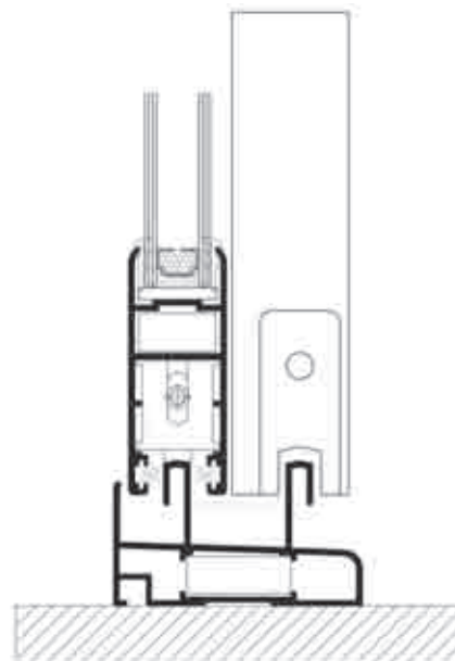
Corredera Samblex P65CO
