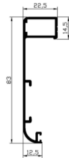
Ref. 121377 Semi marco exterior pared 60
