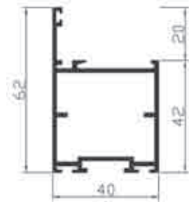
Ref. 19635 Hoja
