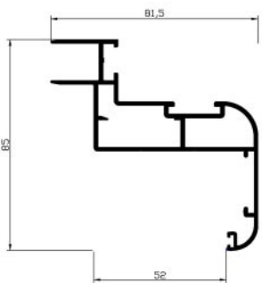
Ref. 121378 Semi marco interior pared 60
