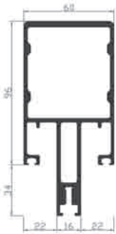
Ref. 21106 Montante
