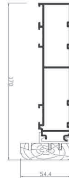
Ref. 21905+7L2 Marco lateal corredera elevable
