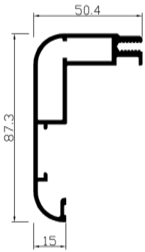
Ref. 121581 Semi marco exterior
