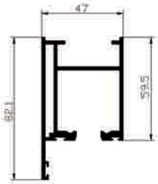
Ref. 19643 Guía superior
