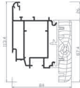
Ref. 21912+7L0 Hoja balconera
