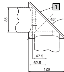
1 Placa desmontable 75 x 174 mm
