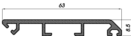
LC28 Terminale in gomma
