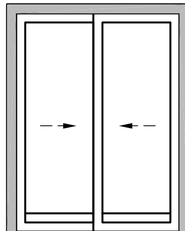
PFin. Scorrevole L= 1300-2800mm H= 1800-2450mm
