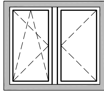
Fin. 2 ante L= 750-1800mm H= 600-1800mm
