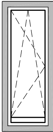
PFin. 1 ante L= 500-1100mm H= 1800-2450mm
