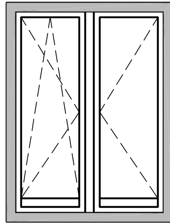
PFin. 2 ante L= 900-1800mm H= 1800-2450mm
