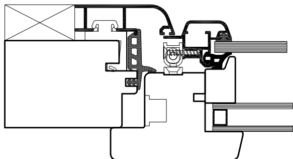
Sistema Verbund Soft-Line/45
