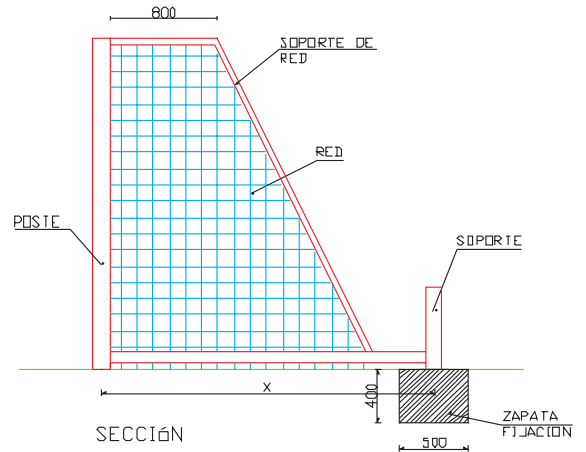
PORTERIA ABATIBLE PF 7ABA PF 7ABM
