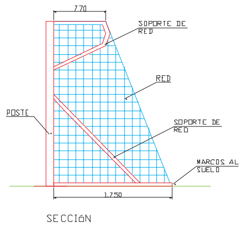
PORTERIA ABATIBLE PF 7ABA PF 7ABM
