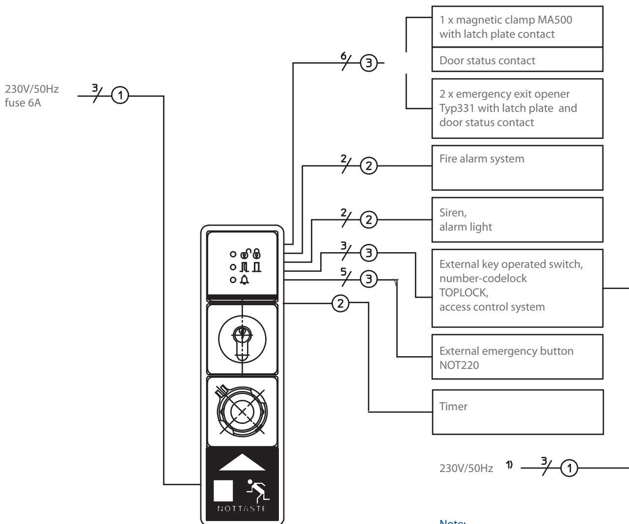
Fig. 04-1 · Cable diagram ((Drawing No. 35201-9-0952)
