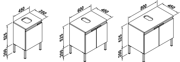
LOS MUEBLES EMMA BASIC SE SUMINISTRAN DESMONTADOS (MODULO ARMAZÓN / KIT ENCIMERA + PUERTAS) EMMA BASIC FURNITURES ARE DELIVERED UNMOUNTED (FRAMEWORK / OVERCOUNTER KIT + DOORS)
