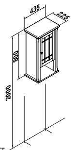
VITRINA # 38660 WALL MOUNTED CABINET
