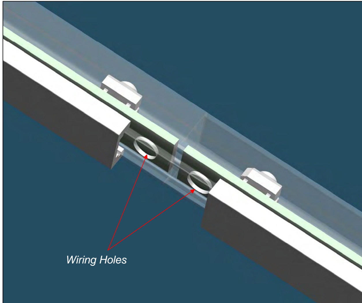
Rear View LEDFLOODSTRIP 45 LED's/m
