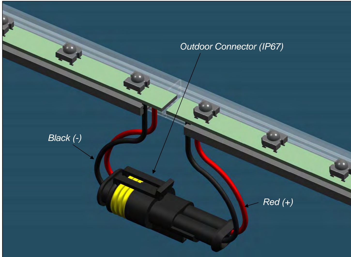
Connection View LEDFLOODSTRIP 45 LED's/m
