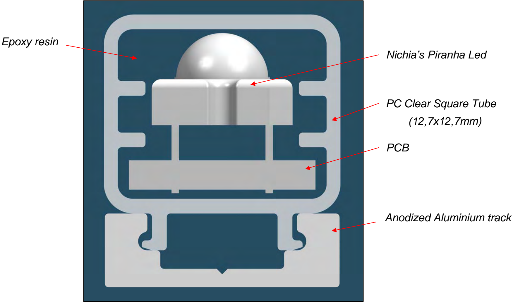
Side View LEDFLOODSTRIP 45 LED's/m
