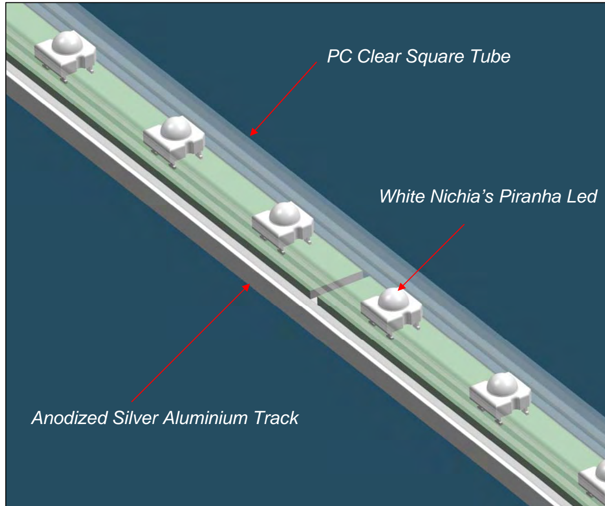
General View LEDFLOODSTRIP 45 LED's/m (180 Lumens information from Data sheet Nichia)
